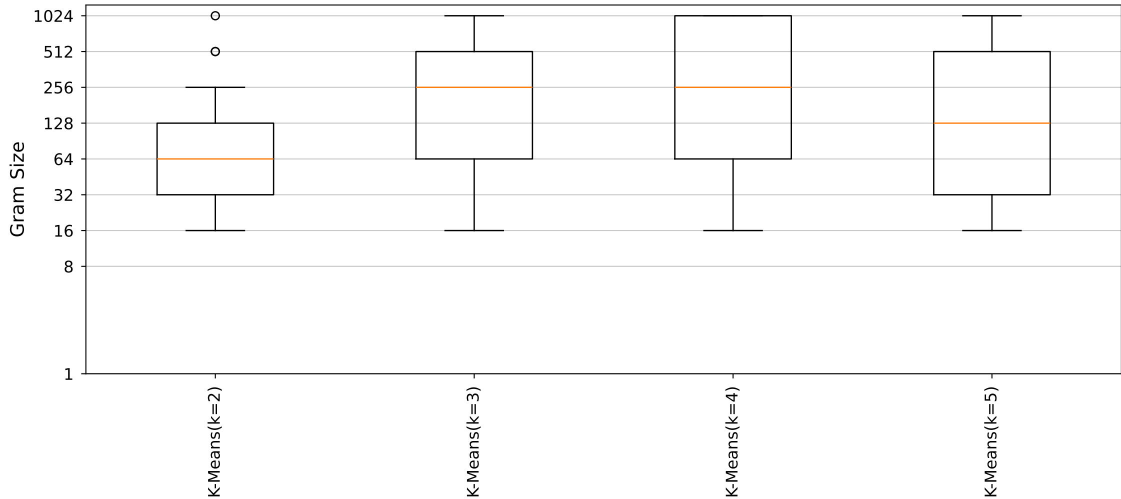
YARA Rules Gram Size Distribution (Cluster44_Size5 dataset)
